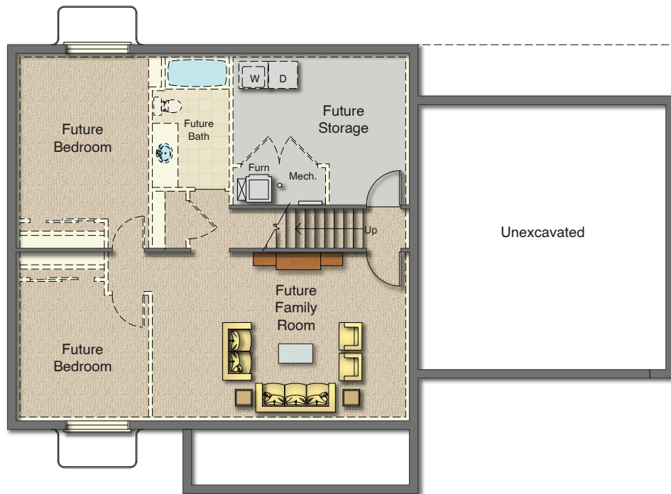
Standard Basement - 960 Sq.Ft.
