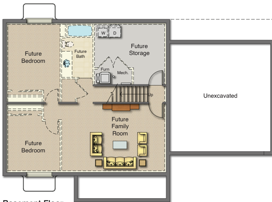
Basement Floor 960 Sq.Ft.
